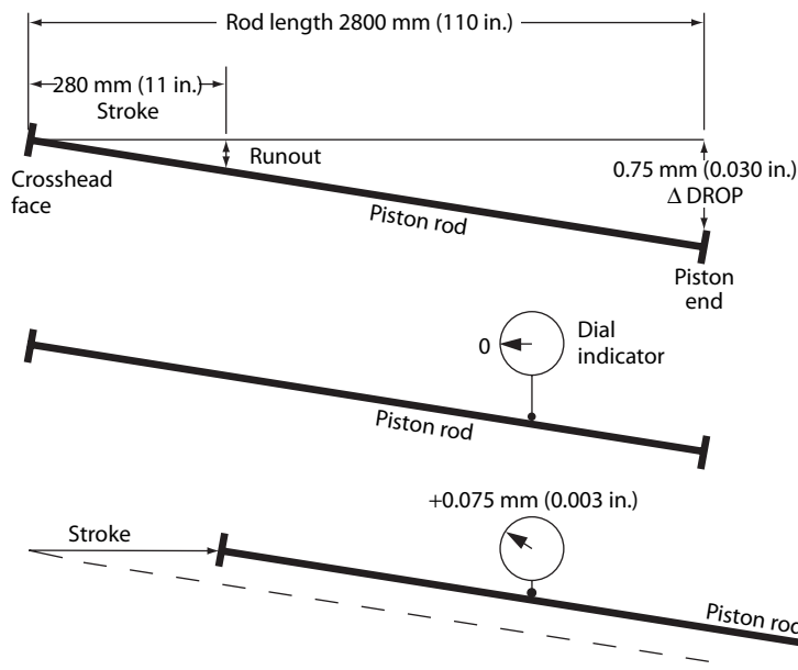
Figure C-2—Vertical Runout Geometric Relationships Based on No Rod Sag
